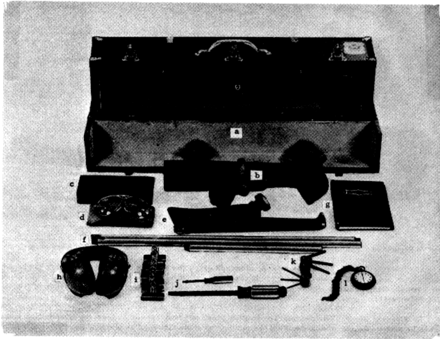
Figure 11. Shooting box and accessories.
